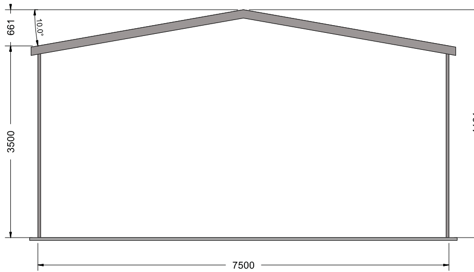
FRONT ELEVATION
