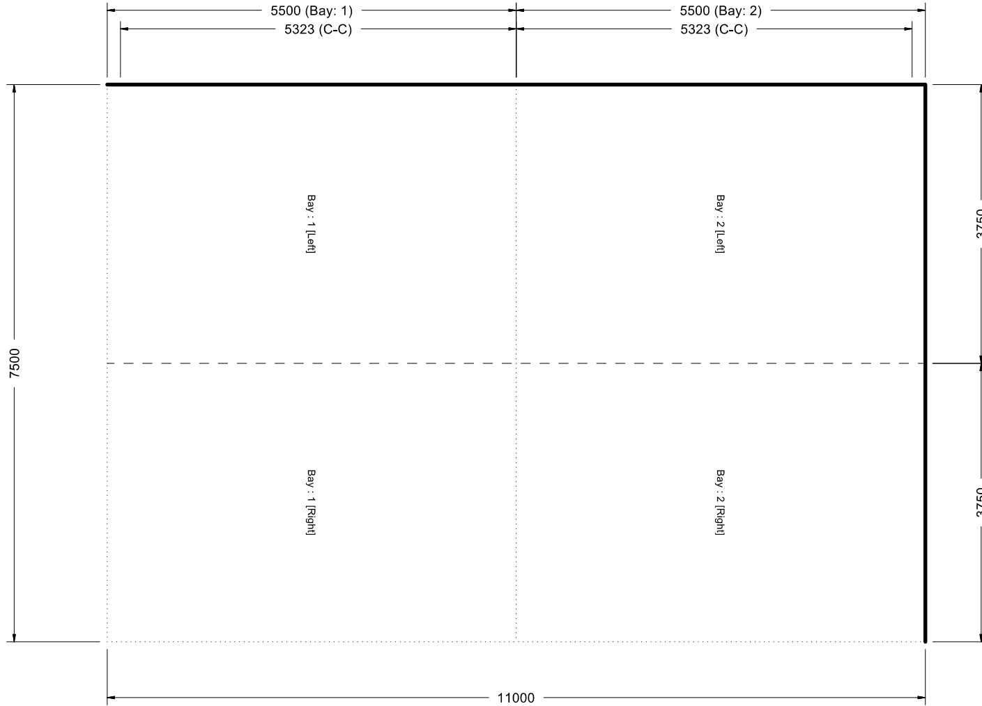
PLAN ELEVATION
