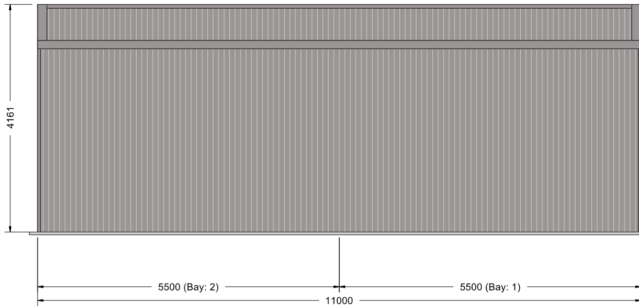
LEFT ELEVATION
